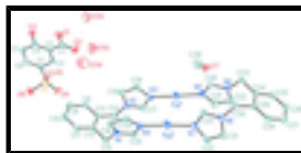
Fig. 1. The asymmetric unit of the title compound, showing the atomic numbering scheme. Displacement ellipsoids are drawn at the 30% probability level. Only the major disorder component of the \text{C}_7\text{H}_4\text{O}_6\text{S}^{2-} ion is shown.
